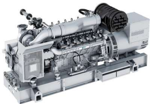
SGE-42HM genset.
